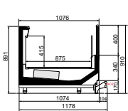
Whale 2000 G MT - HG400
