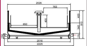
Whale 2000 G - HG400
