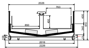
Whale 2000 G 2EV - HG400
