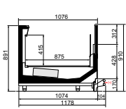
Whale 2000 G MT - LG300
