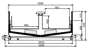
Whale 2000 G 2EV - LG300
