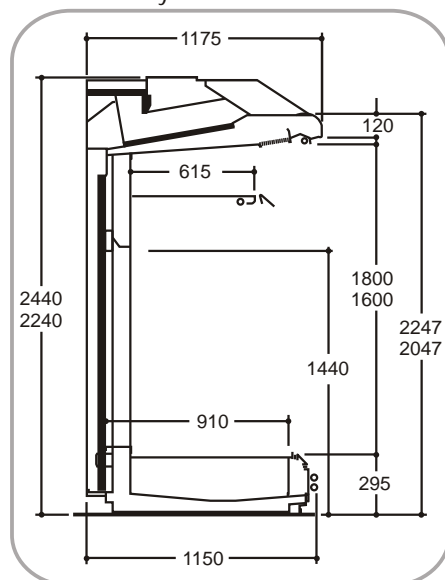
Impala back loading H20-22 Trolley
